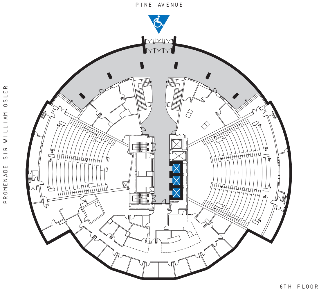
6TH FLOOR
